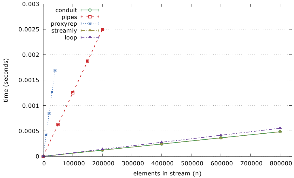
Fig. 8. Results of the fold micro-benchmark.
