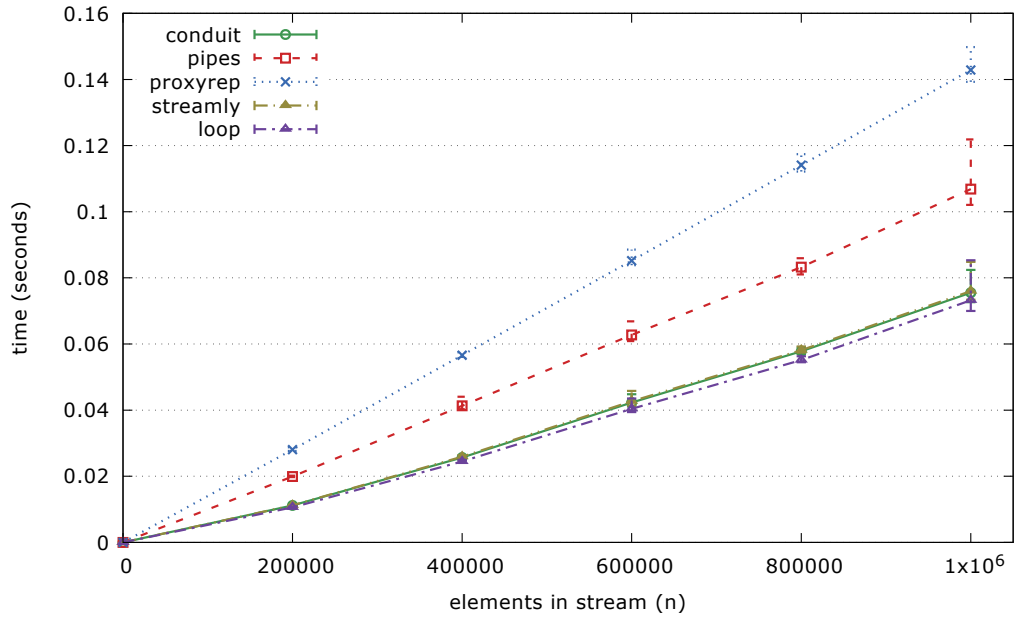
Fig. 5. Results of the mapM micro-benchmark.
