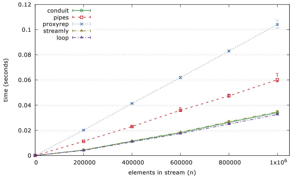
Fig. 6. Results of the filter micro-benchmark.
