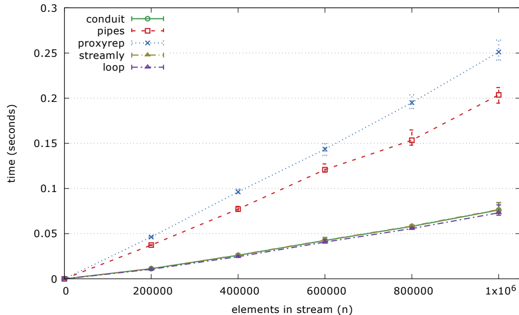
Fig. 4. Results of the map micro-benchmark.
