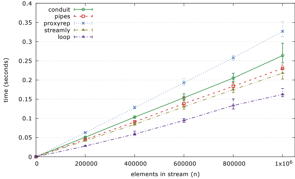
Fig. 7. Results of the concat micro-benchmark.
